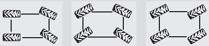
2 WHEEL STEERING
